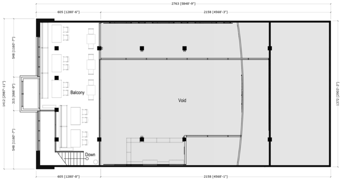
2nd Floor Plan Micro Brewery Scale 1 : 100
