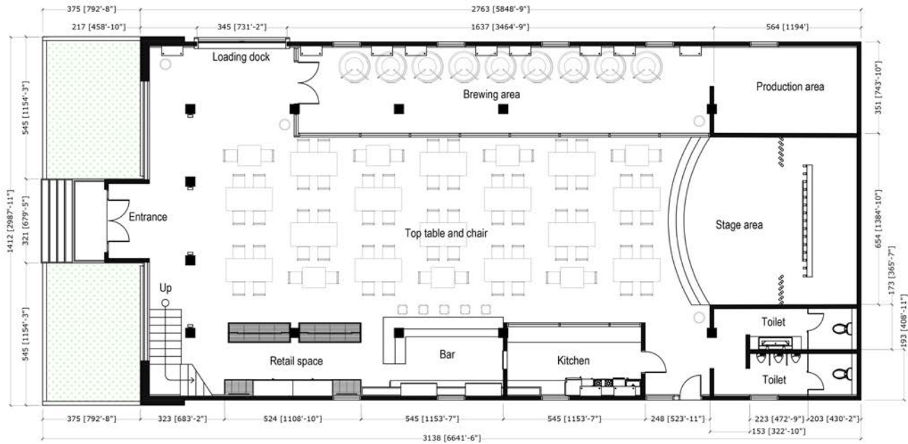
1st Floor Plan Micro Brewery Scale 1 : 100
